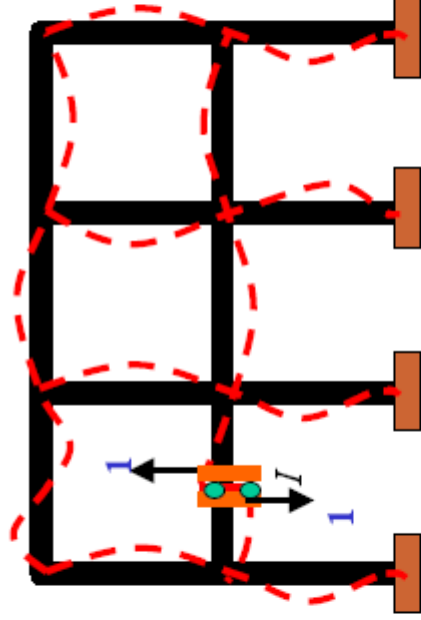
Influence Line of V_1
